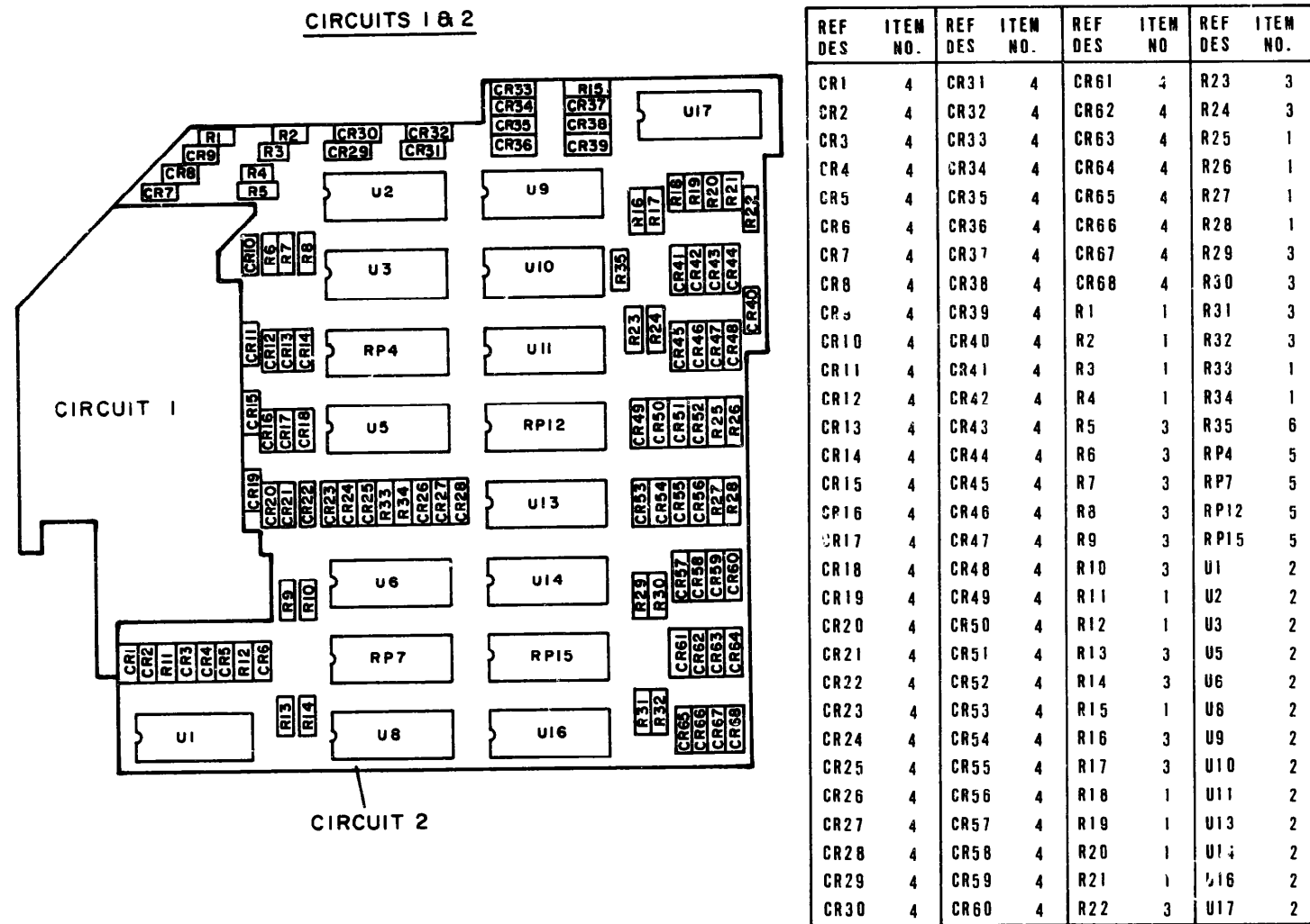
Figure 29. Circuits 1 and 2 of Circuit Card Assembly 103998-001.
