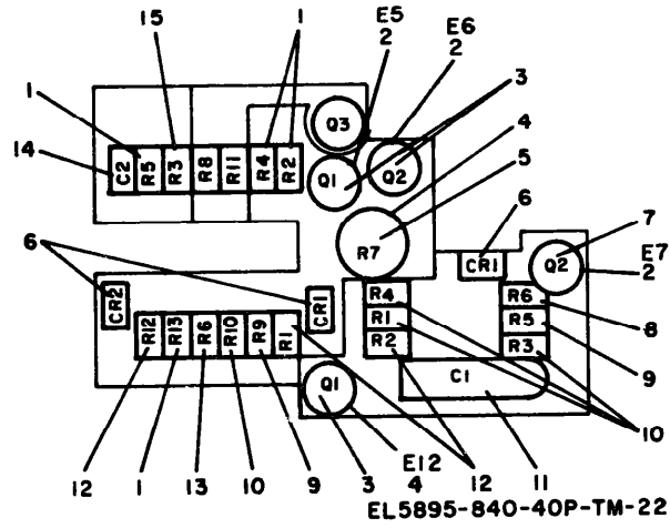
Figure 22. Circuits 18 and 19 of Circuit Card Assembly 104125-003.
