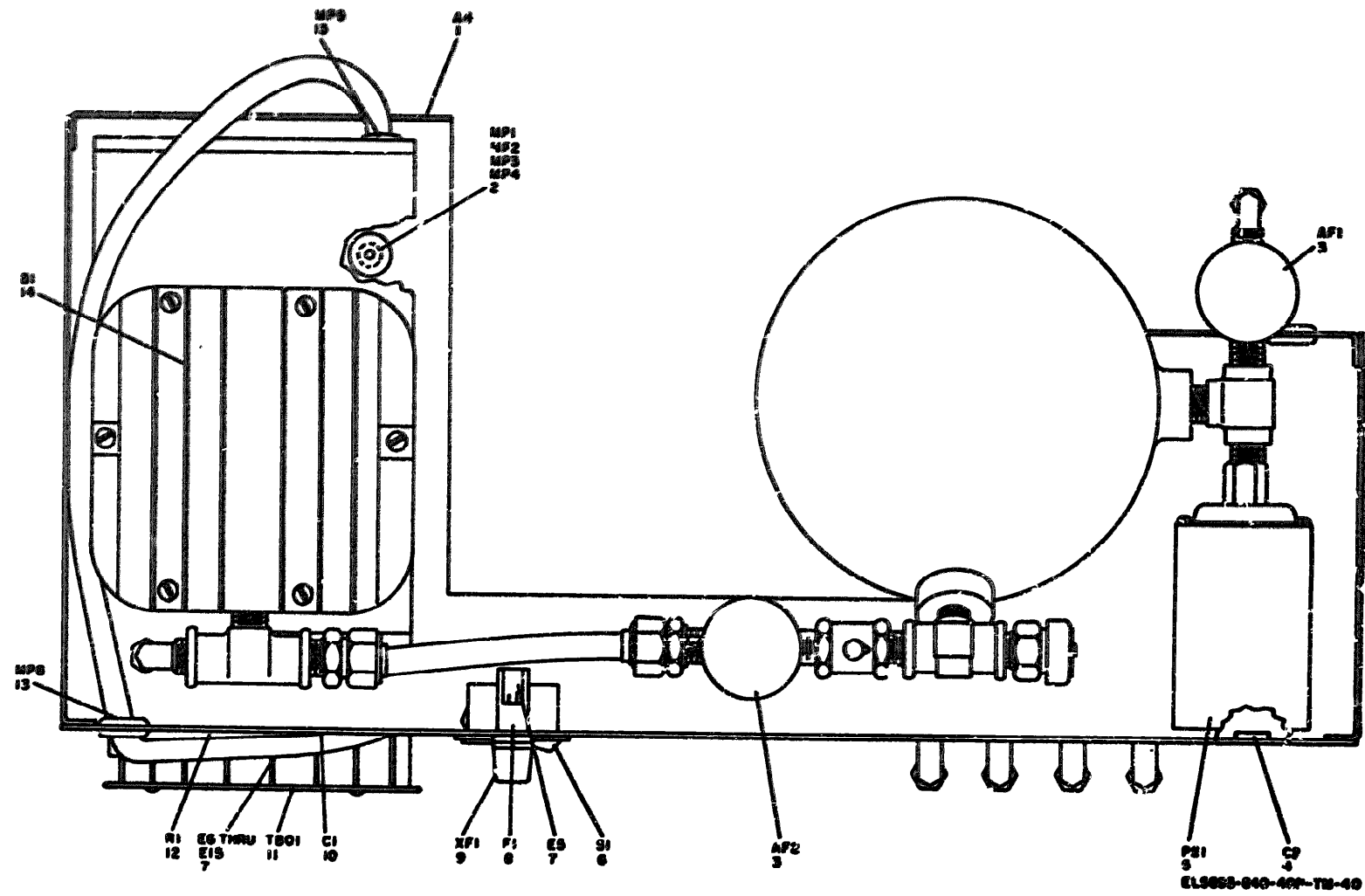
Figure 40. Pneumatic Supply Assembly 106639-001.
