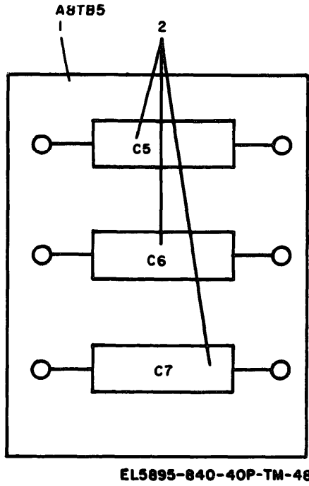
Figure 48. Circuit Card Assembly 103389-001 (Input Line Filter).
