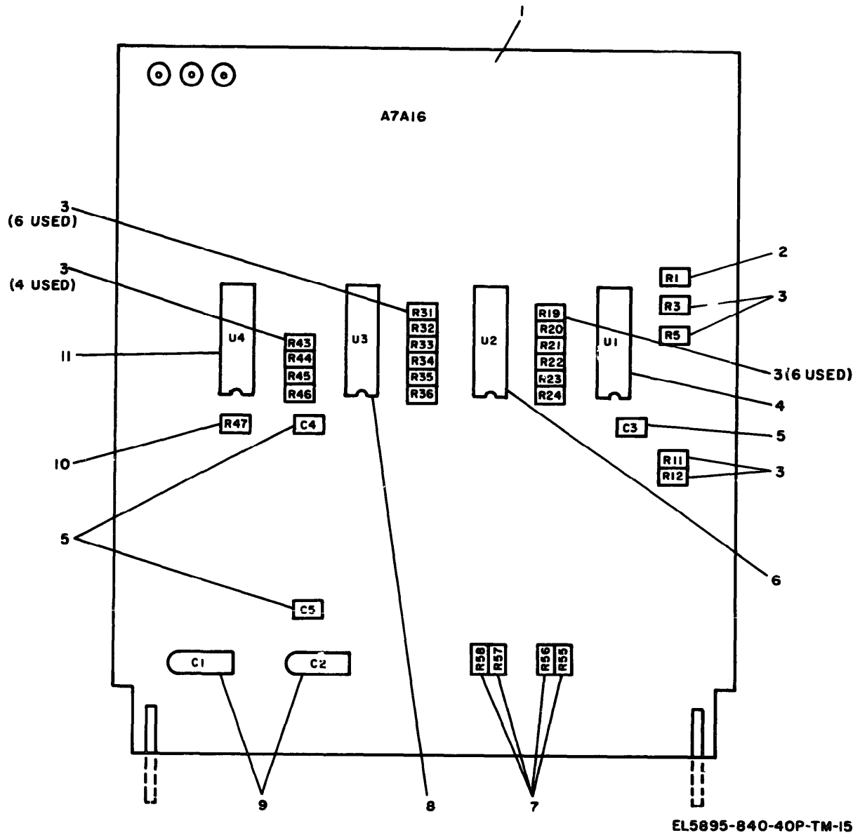
Figure 15. Circuit Card Assembly, 103996-001 (PC, Data Control, PF).
