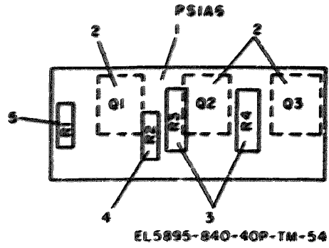
Figure 54. Circuit Card Assembly 100272-001.
