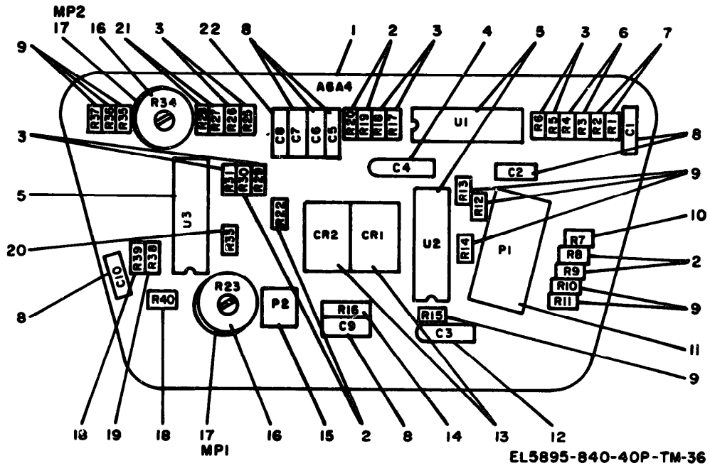
Figure 36. Circuit Card Assembly 104104-001 (PC, Index Sector Detector, PF).
