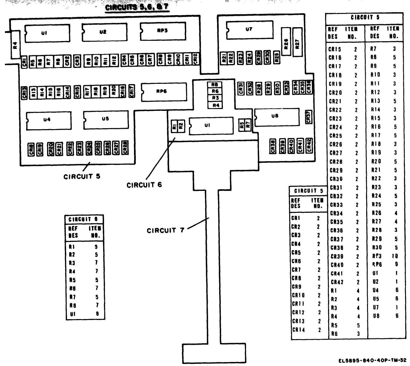
Figure 32. Circuits 5, 6, and 7 of Circuit Card Assembly 103998-001.
