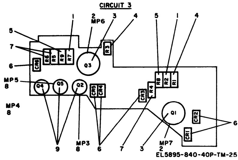
Figure 25. Circuit 3 of Circuit Card Assembly 104141-001.
