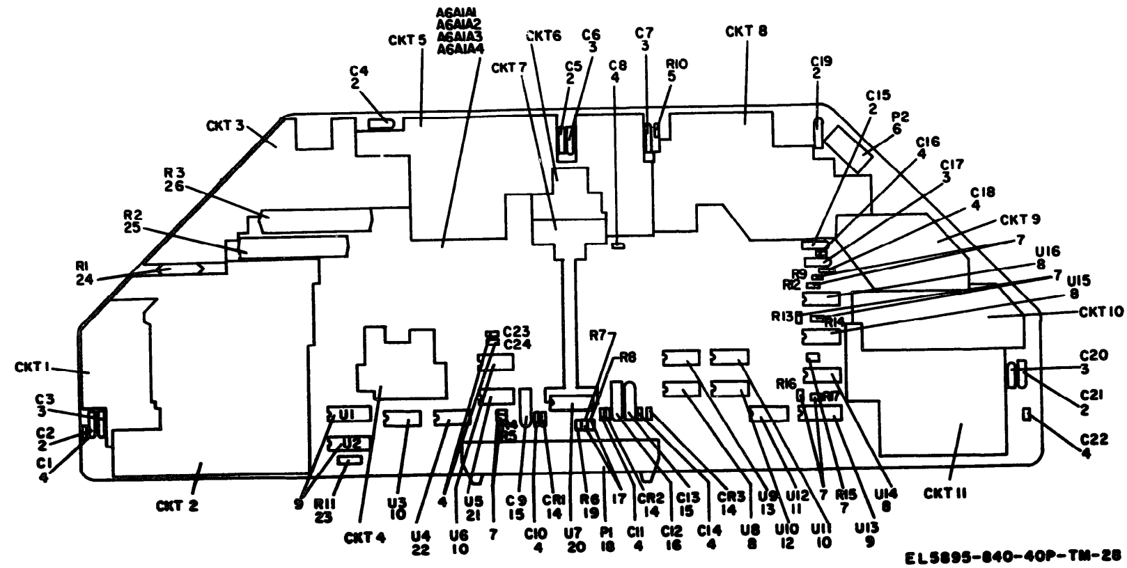
Figure 28. Circuit Card Assembly 103998-001.
