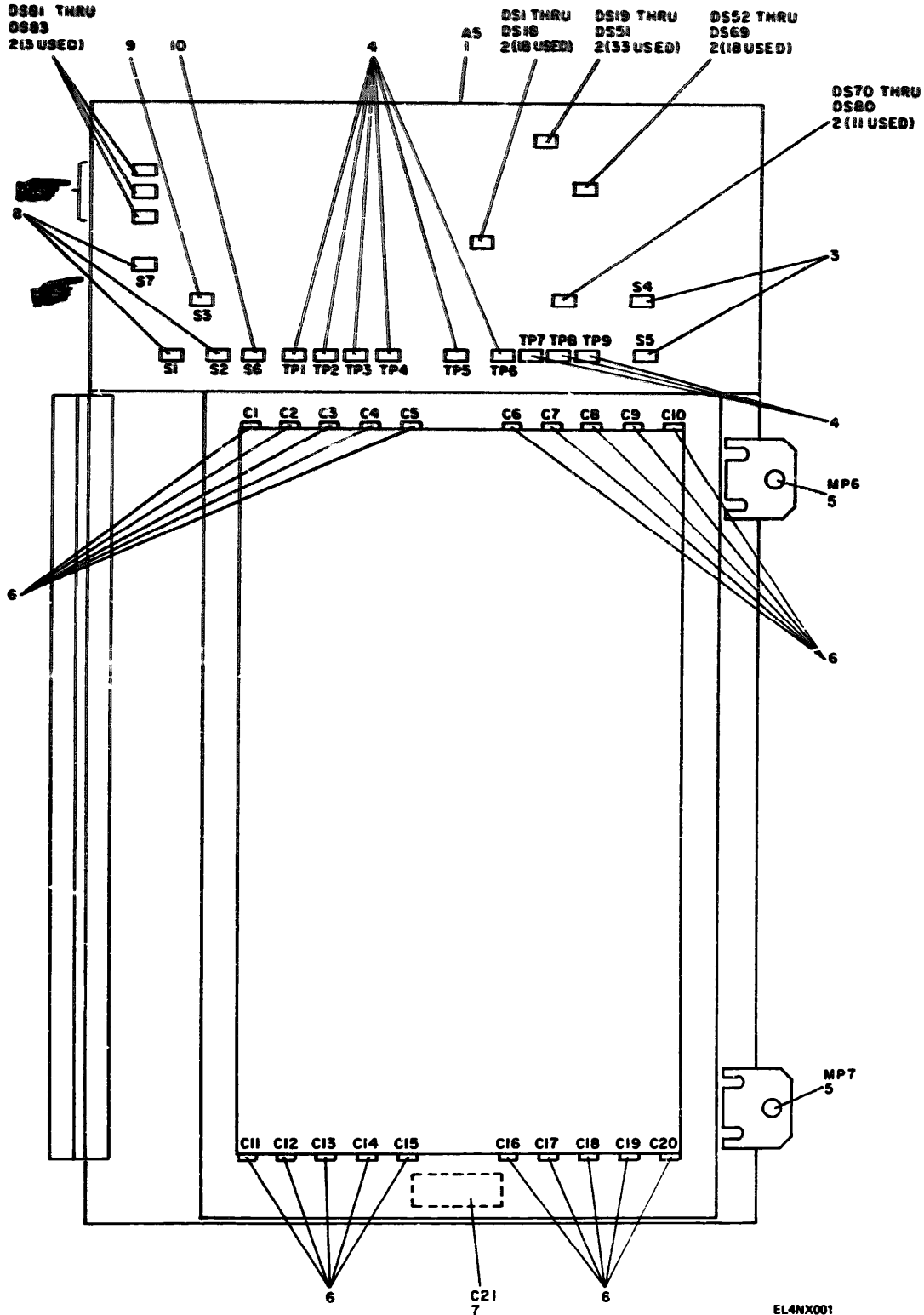
Figure 1. Disc Controller, Parts Location.
