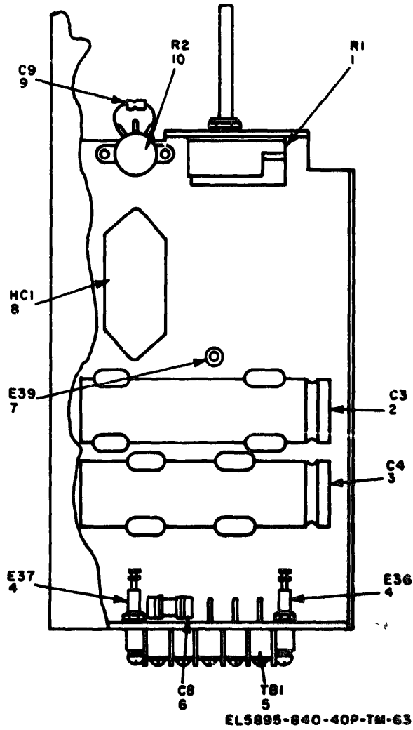
Figure 63. Power Supply PP-7144/U LXSD5-OV, Side Cutaway View.
