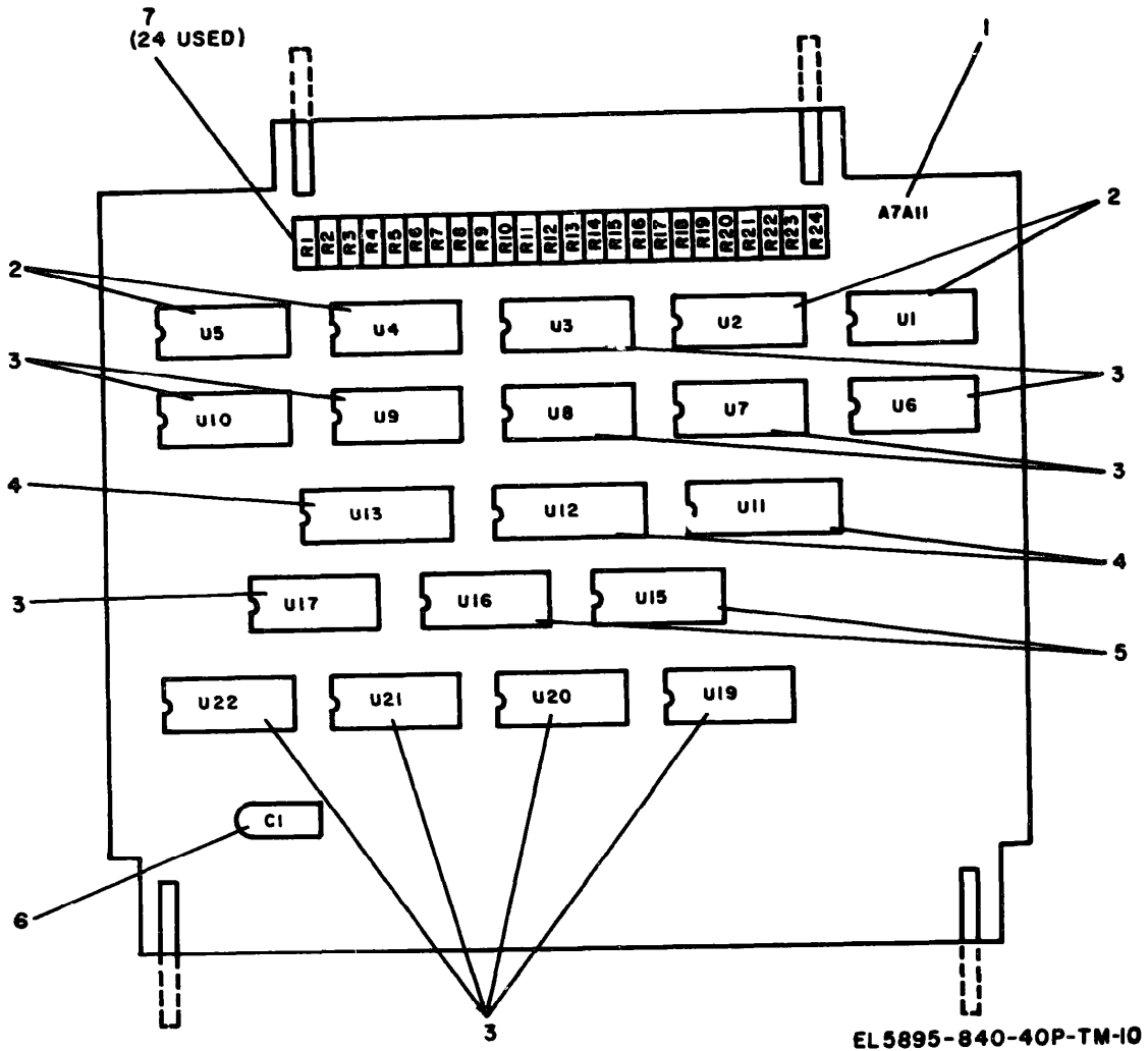
Figure 10. Circuit Card Assembly, 103990-001 (PC, Spare Select 2, PF).
