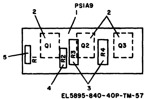
Figure 57. Circuit Card Assembly 100276-001.
