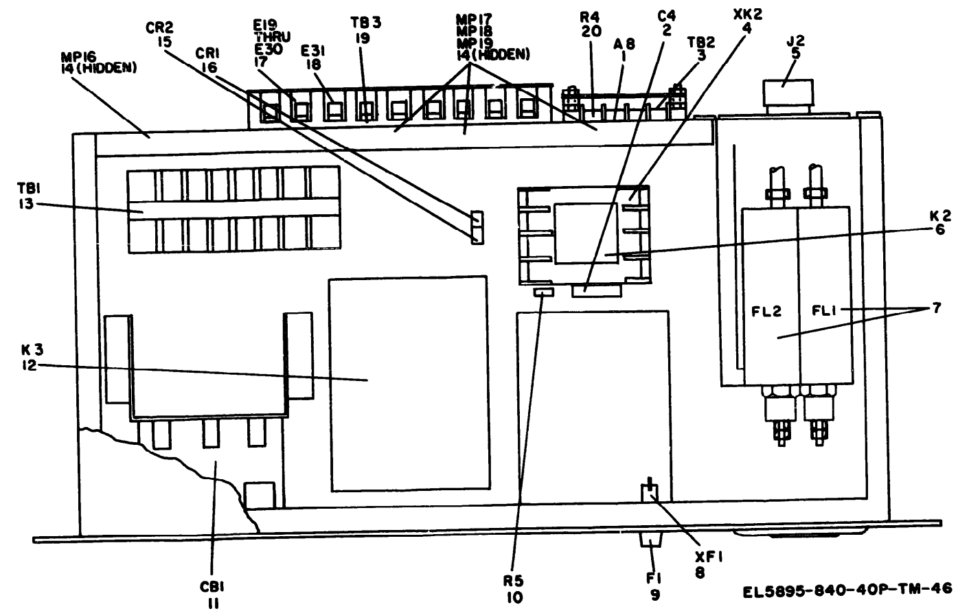
Figure 46. Ac Distribution Chassis Assembly 104028-001.
