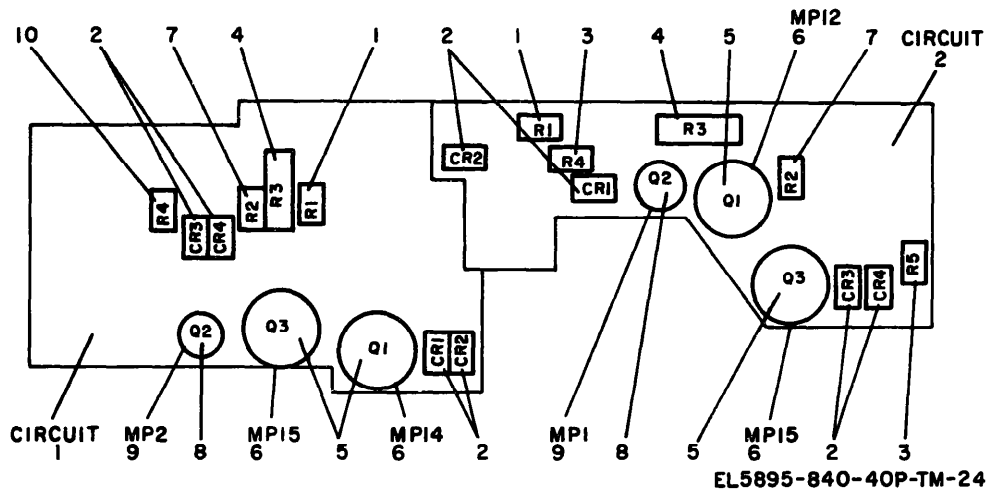
Figure 24. Circuits 1 and 2 of Circuit Card Assembly 104141-001.
