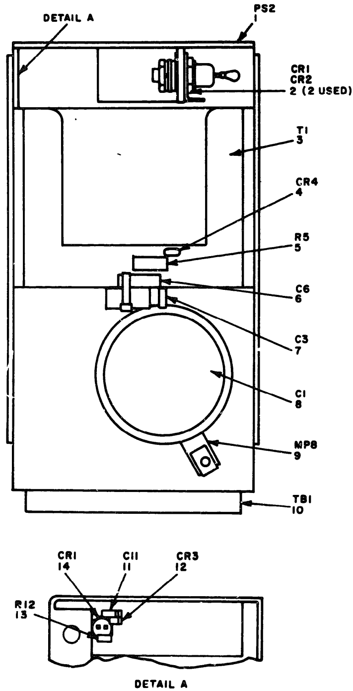
Figure 59. Power Supply PP-7147/U LXSA5-OV.
