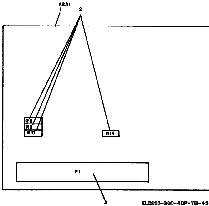
Figure 45. Circuit Card Assembly 104002-001 (PC, Component Board Panel PF).
