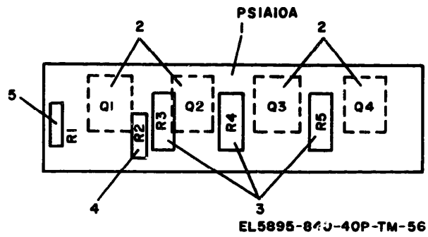
Figure 56. Circuit Card Assembly 100274-001.
