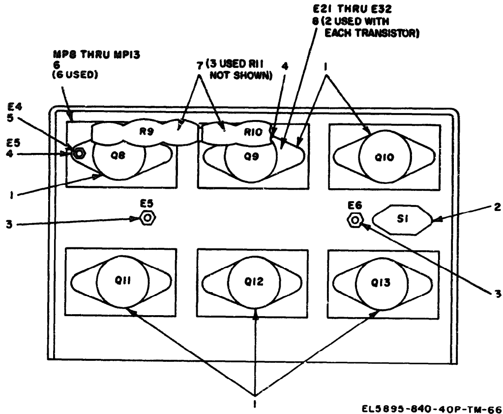
Figure 66. Power Supply PP-7144/U LXSD5-OV, Interior Side View.
