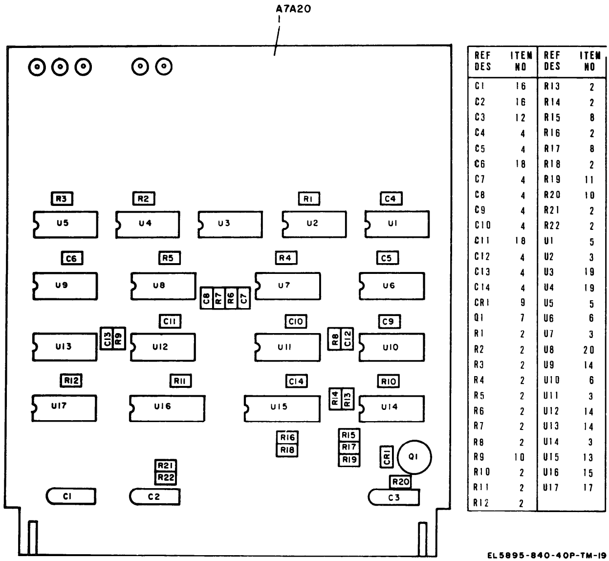
Figure 19. Circuit Card Assembly 103854-001 (Sector Counter, PF)
