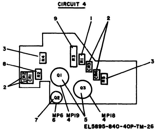
Figure 26. Circuit 4 of Circuit Card Assembly 104141-001.
