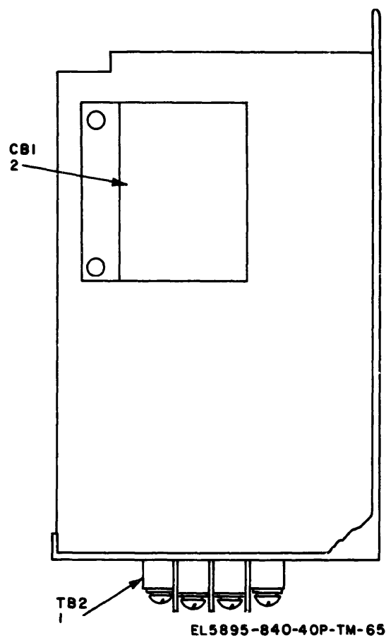
Figure 65. Power Supply PP-7144/U LXSD5-OV, Rear Panel.
