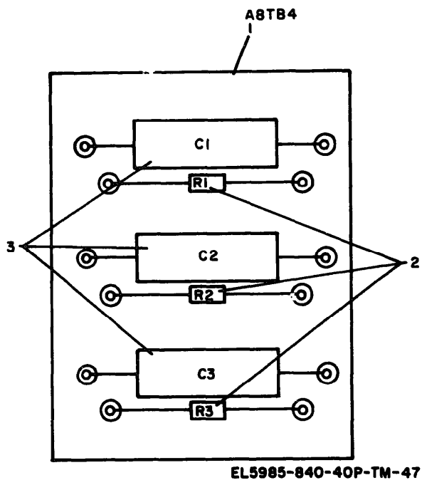
Figure 47. Circuit Card Assembly 103208-001 (Noise Filter).
