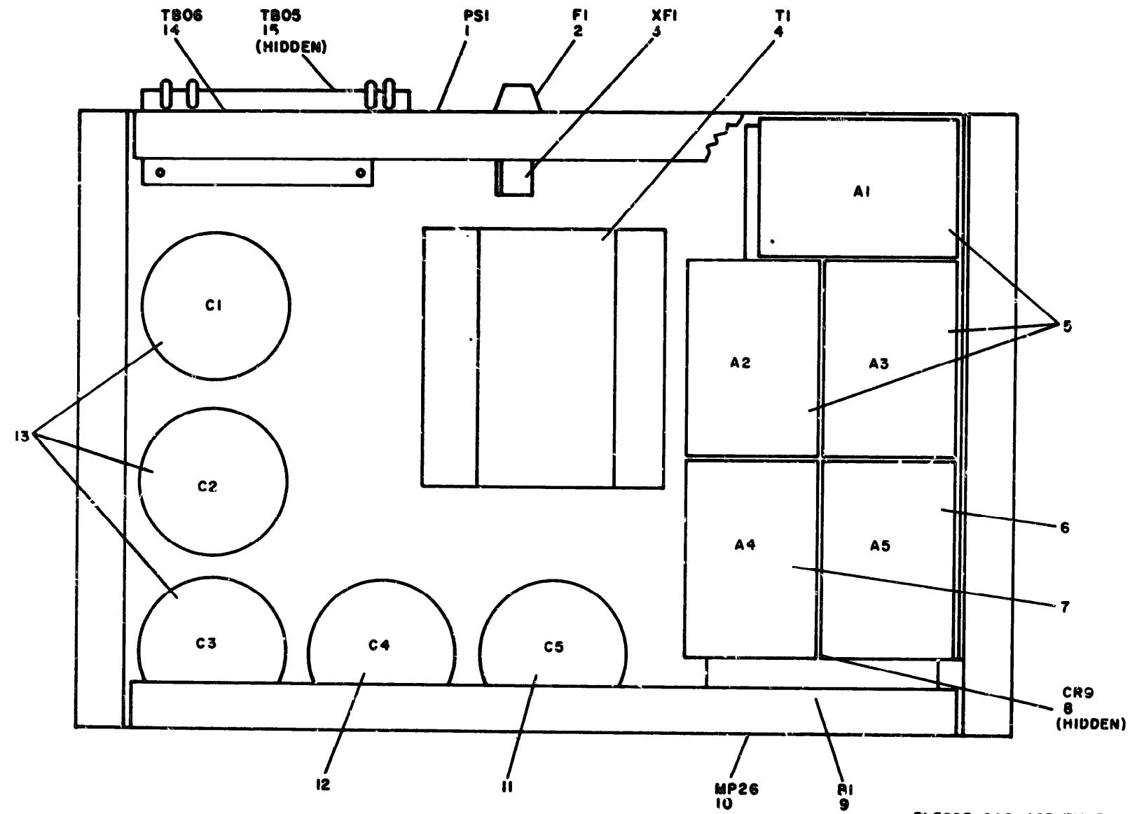
Figure 51. Power Supply 103188-001.
