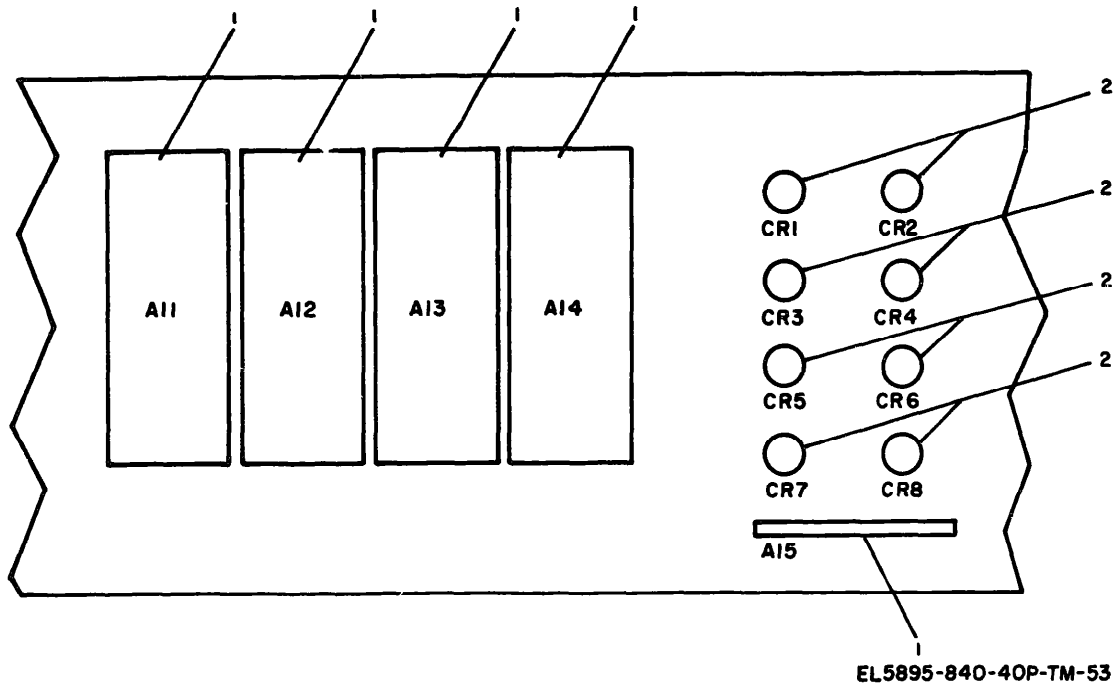
Figure 53. Power Supply Circuit Card Assembly 100275-001 (Bottom Heat Sink View).
