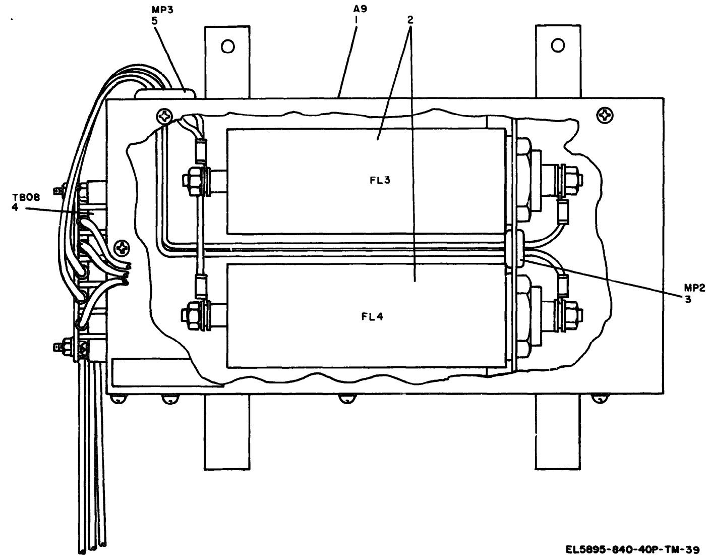
Figure 39. Line Filter Assembly 104038-001.
