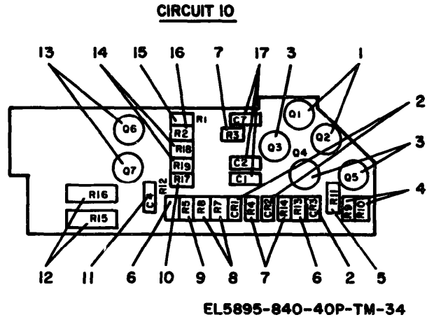
Figure 34. Circuit 10 of Circuit Card Assembly 103998-001.
