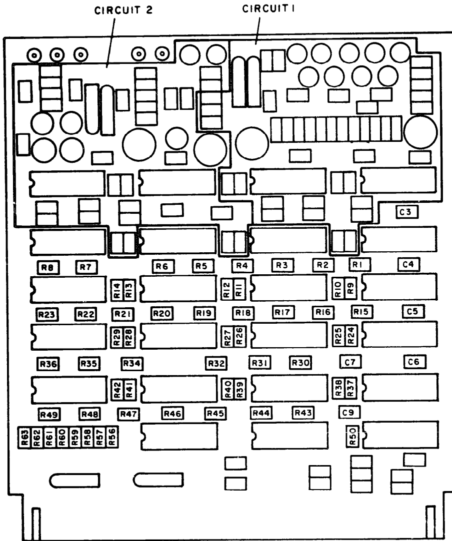
Figure 12. Circuit Card Assembly, 1040700-001, (PC, Read Decode, PL, Diff. Input)
