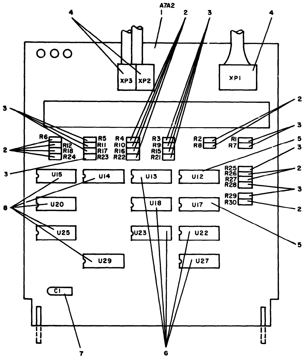
Figure 7. Circuit Card Assembly, 103994-001 (Interface BP, PF).
