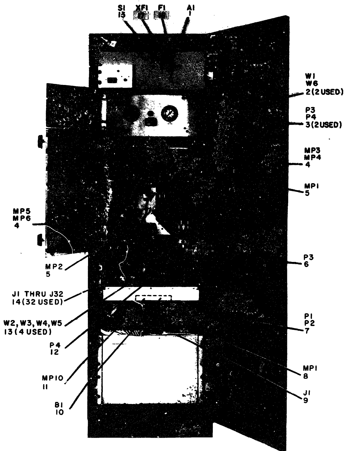
Figure 4. Disc Assembly, 103924-001, Front View
