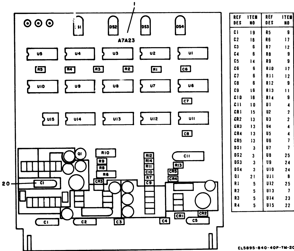
Figure 20. Circuit Card Assembly 104125-003 (PC, U-J Headland Drive No. 2, PF).
