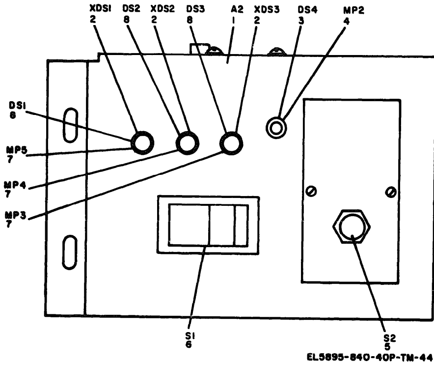
Figure 44. Control Panel Assembly 103984-001.
