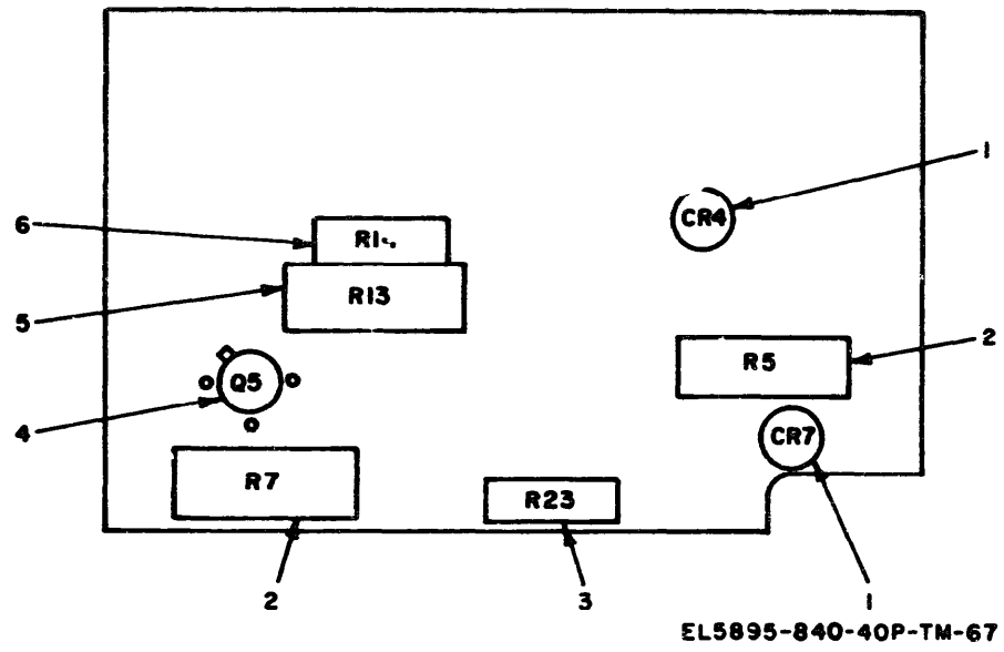
Figure 67. Power Supply PP-7144/U LXSD5-OV, Component Board.
