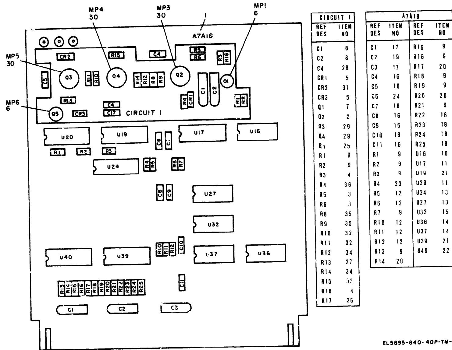
Figure 18. Circuit Card Assembly 104006-001 (PC, Timing Generator, PF).
