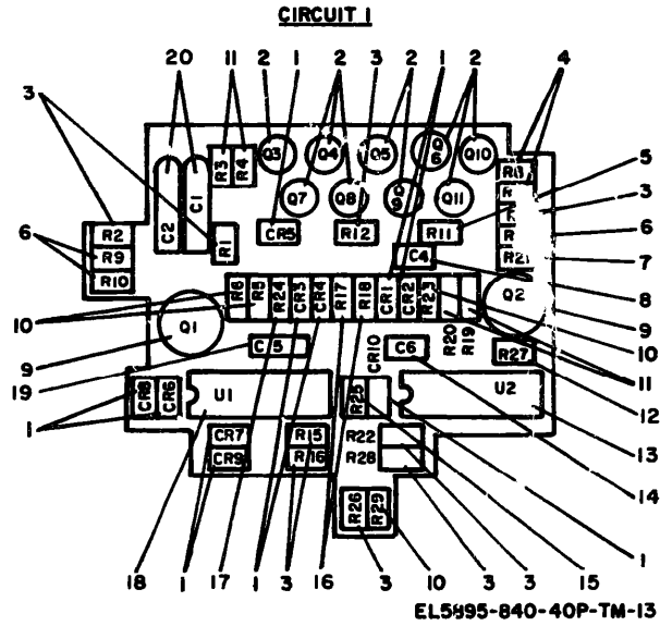
Figure 13. Circuit Card Assembly 104070-001.
