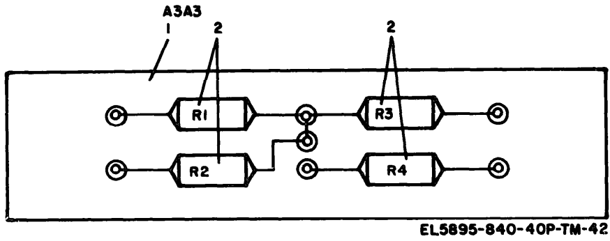
Figure 42. Circuit Card Assembly 103227-001 (Current Reducer).
