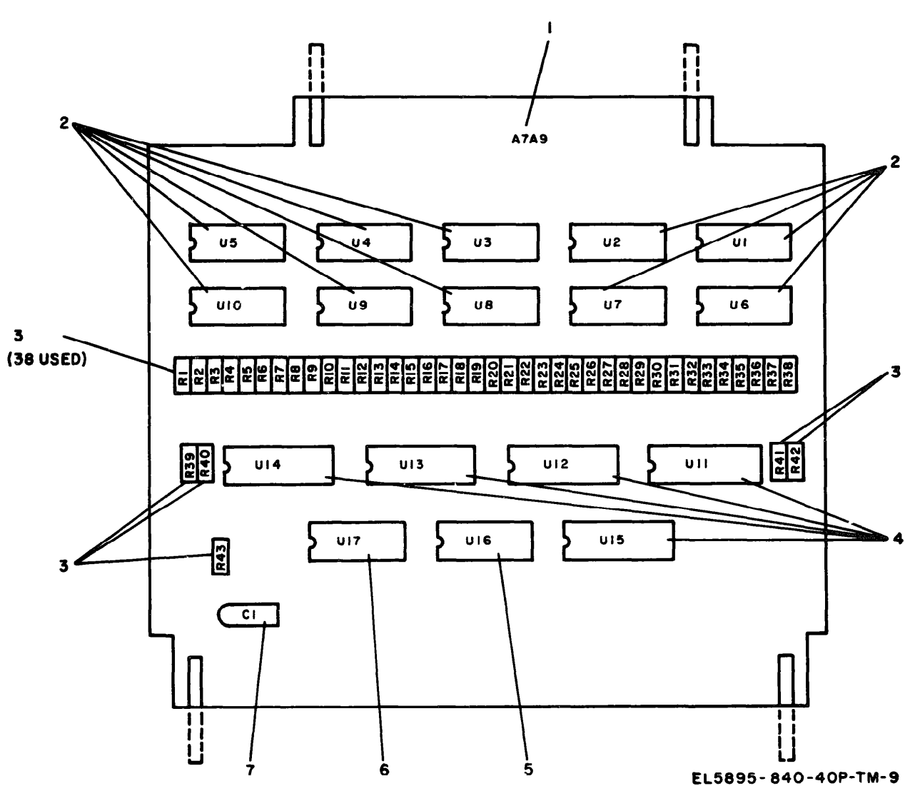
Figure 9. Circuit Card Assembly, 104134-001 (Track Address, PF).
