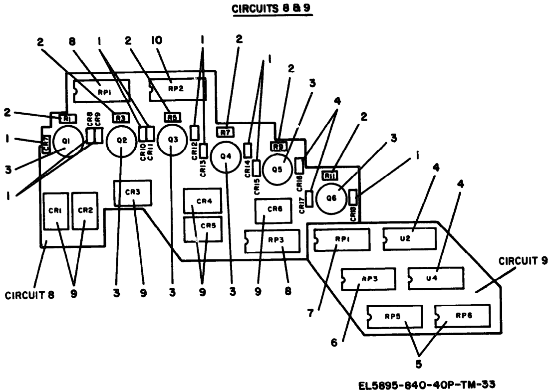
Figure 33. Circuits 8 and 9 of Circuit Card Assembly 103998-001.
