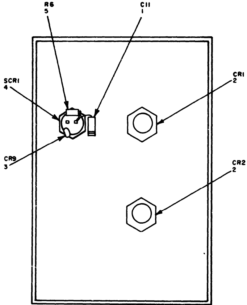
Figure 64. Power Supply PP-7144/U LXSD5-OV, Interior Front Panel.
