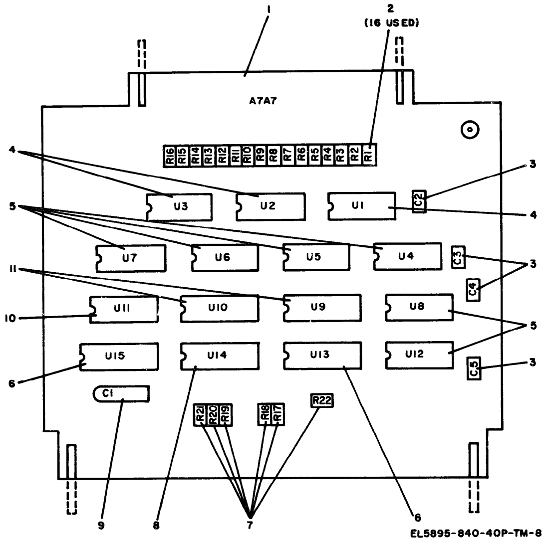
Figure 8. Circuit Card Assembly, 103959-001 (PC, Spare Select, PF).
