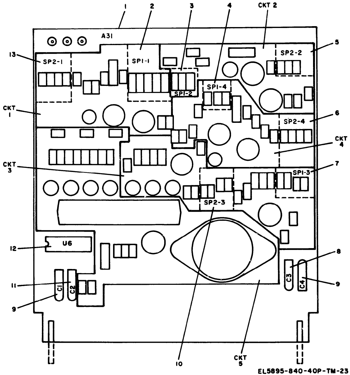
Figure 23. Circuit Card Assembly 104141-001 (Power Present, Clamp, PF).
