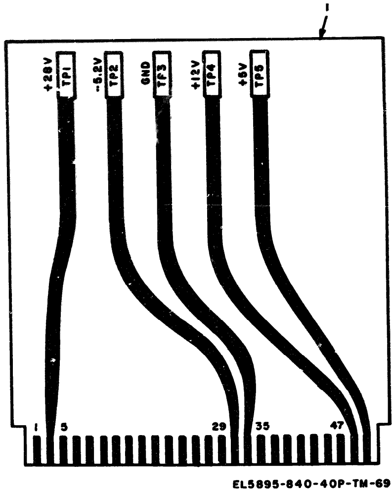
Figure 69. D.C. Voltage Test Board 105397-001.
