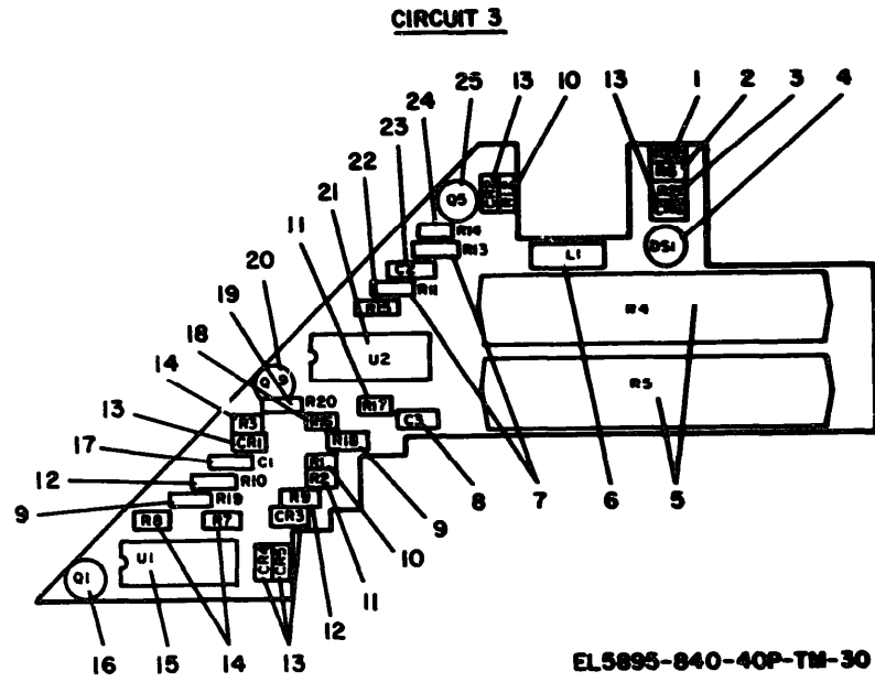
Figure 30. Circuit 3 of Circuit Card Assembly 103998-001.
