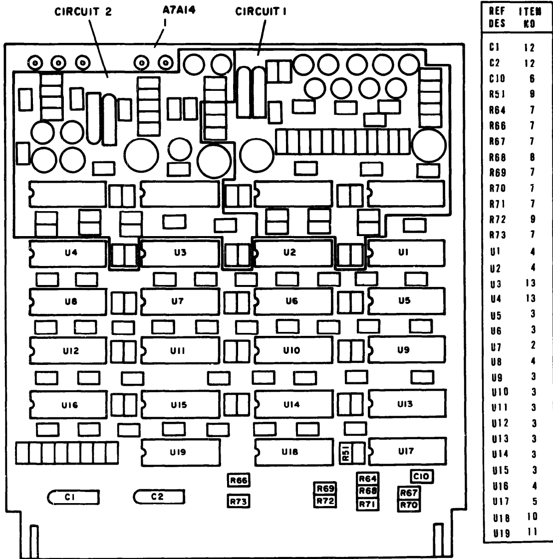
Figure 11. Circuit Card Assembly, 104070-001 (PC, Read Decode, PL, Diff. Input)
