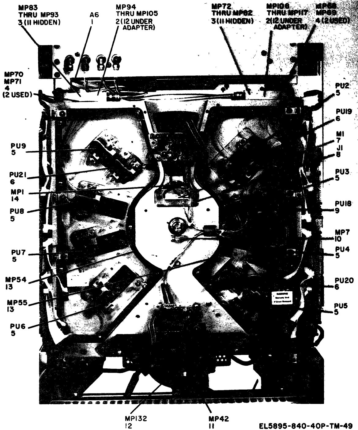
Figure 49. Module Assembly 104305-001, Front View.
