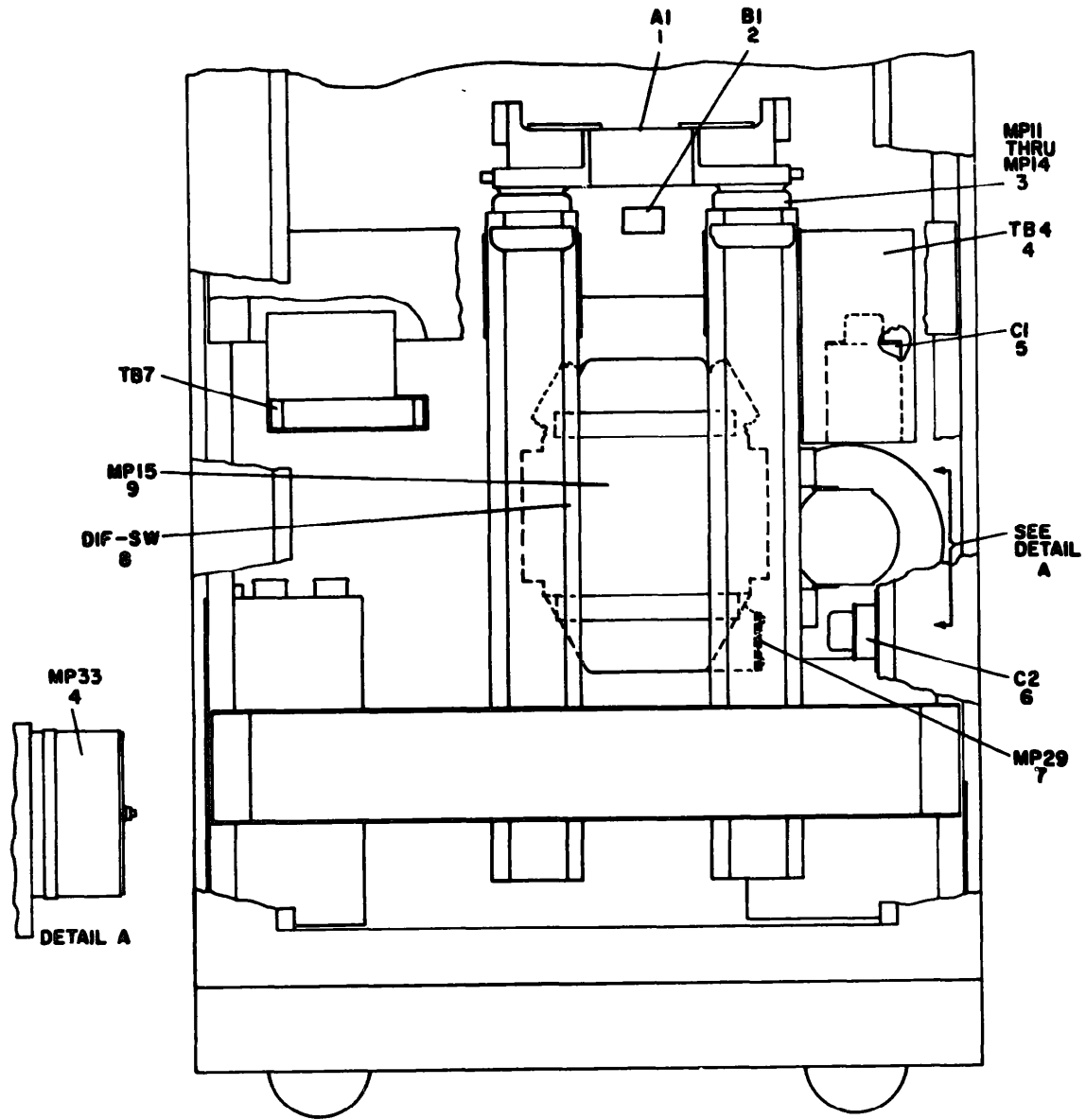
Figure 37. Disc Drive Assembly 103902-001.
