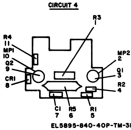
Figure 31. of Circuit Card Assembly 103998-001.
