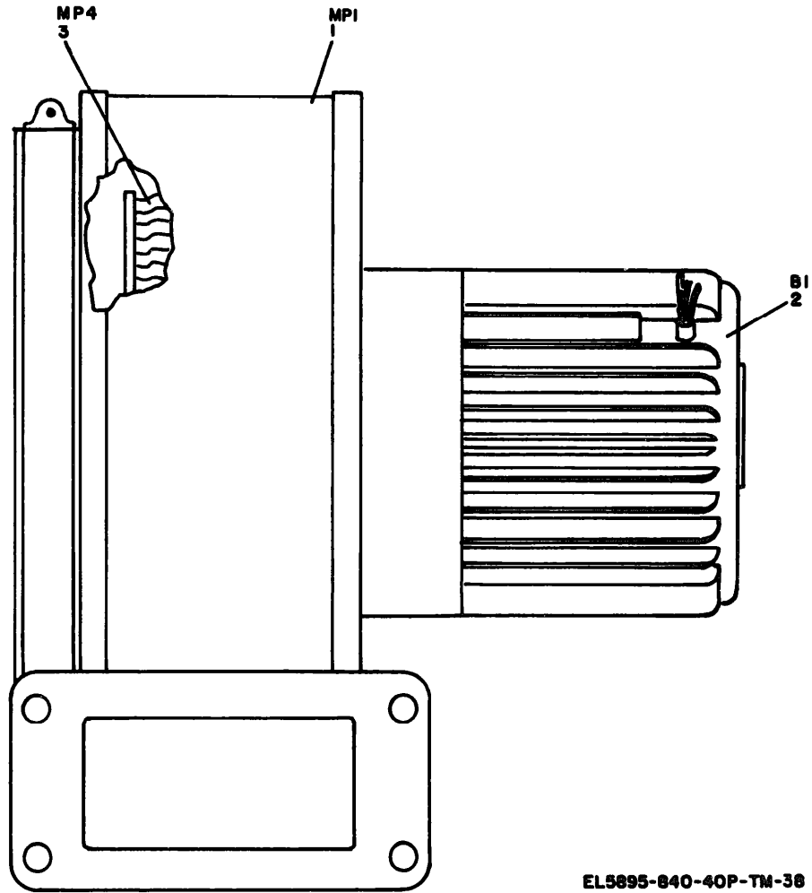
Figure 38. Blower Assembly, Parts Location.
