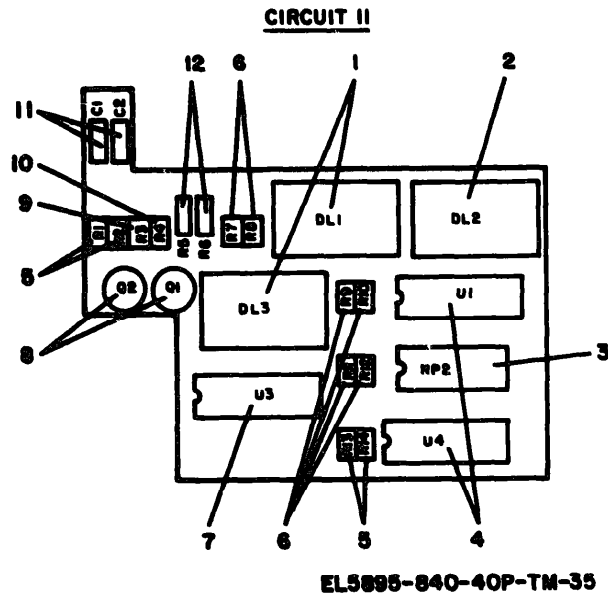
Figure 35. Circuit II of Circuit Card Assembly 103998-001.
