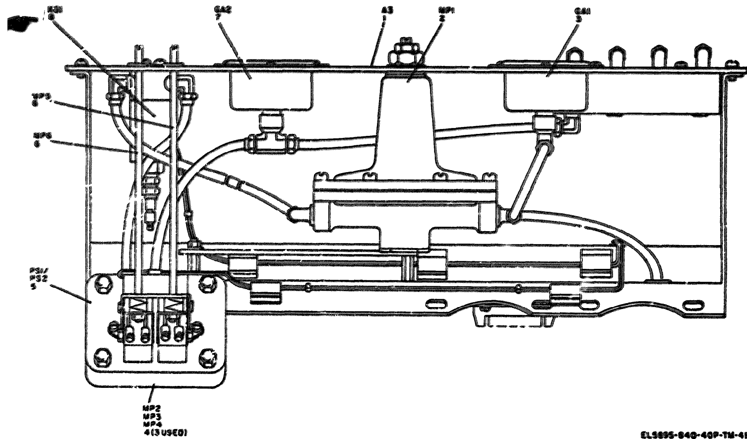
Figure 41. Pneumatic Control Panel Assembly 103883-001.
