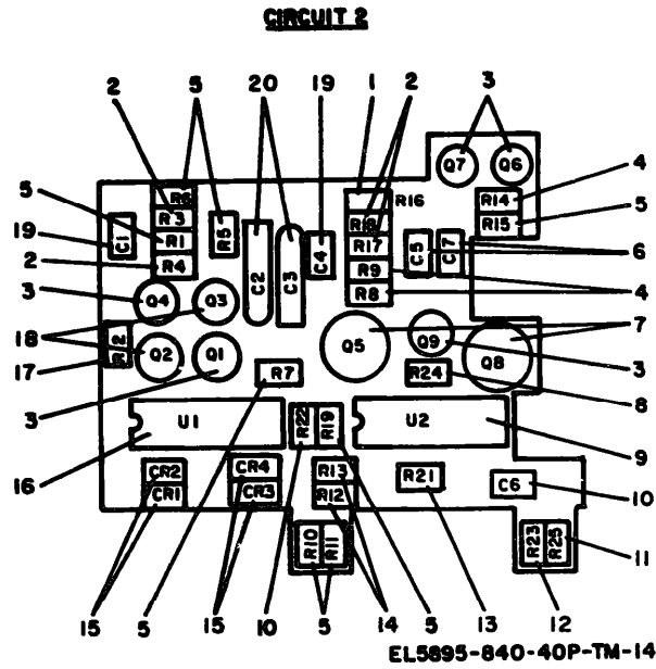
Figure 14. Circuit 2 of Circuit Card Assembly 104070-001.
