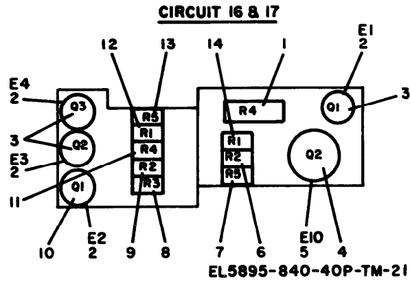
Figure 21. Circuits 16 and 17 of Circuit Card Assembly 104125-003.
